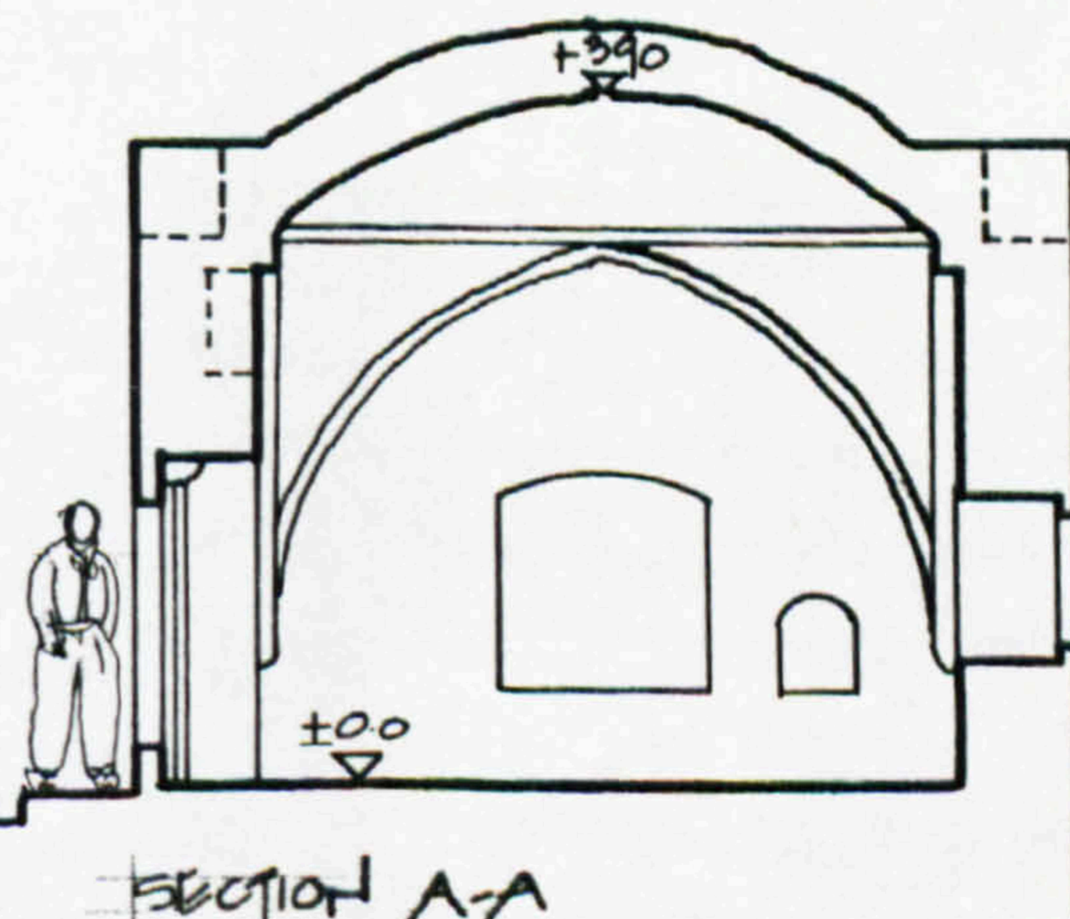
Fig. 4.35 The Shu'aibi Elevated Room ('Allieh)
